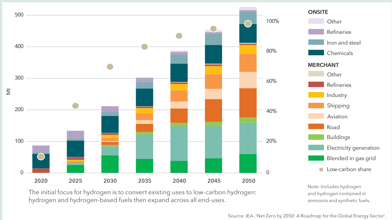
Figure 11: Global H 2 and H 2 -based fuel demand in IEA Net-zero Scenario (IEA, 2021)
