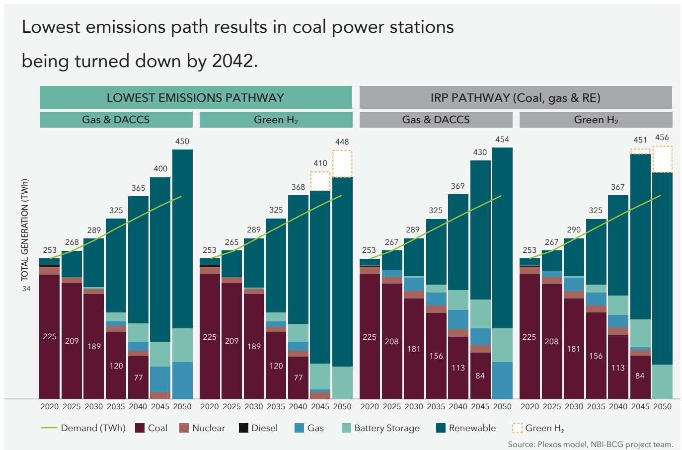
Figure 13: Comparison of generation per technology in the pathways
