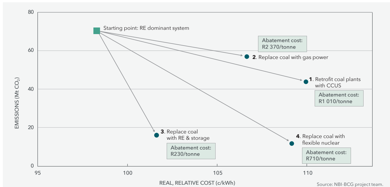
Figure 9: Decarbonisation options for residual emissions
